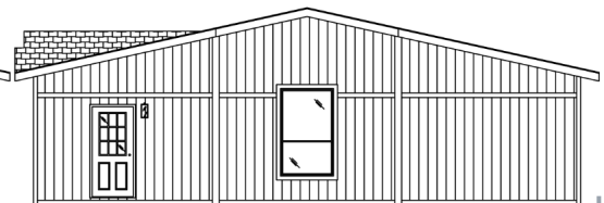
REAR ENDWALL
